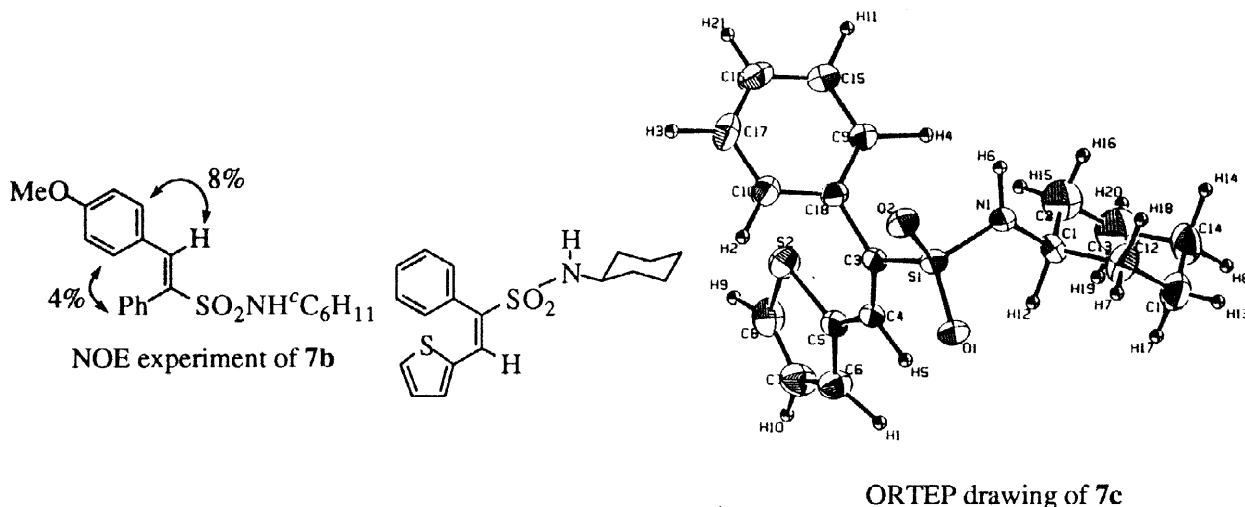
Fig. 1. Structure determination of vinylsulfonamides 7
